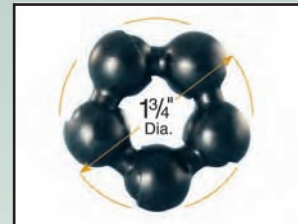
SwivelMax links swivel 72° either side of centerline enabling it to come full circle within a 1 3/4" inscribed circle.
