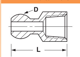
TYPE 4 - Fits 1/8 NPT/BSPT
